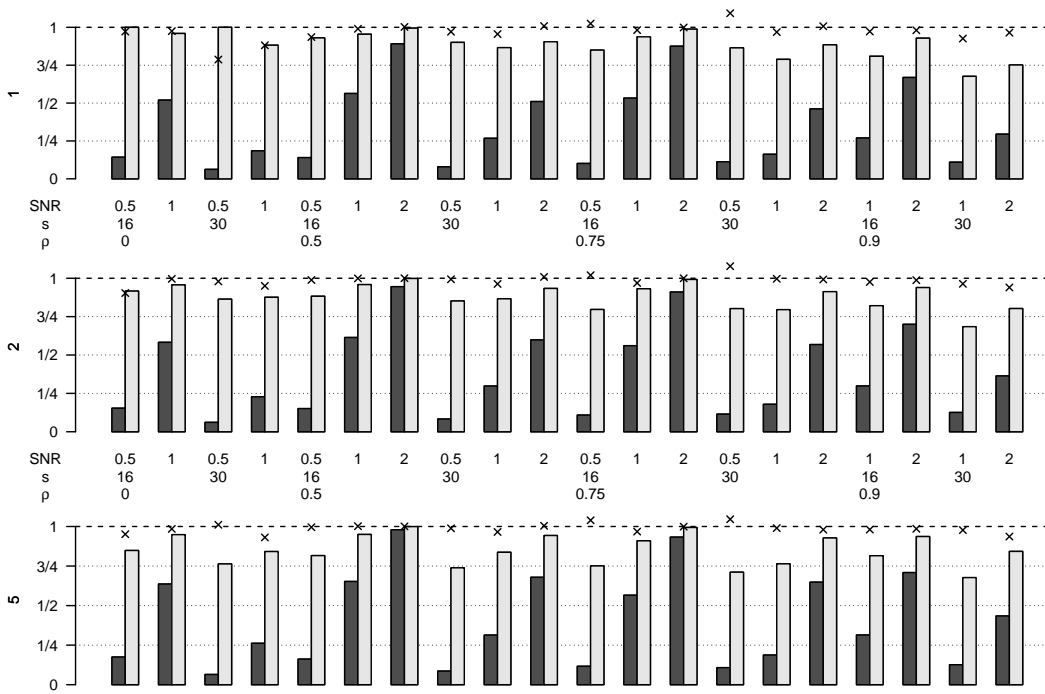
Fig. 5. As above but n = 500 , p = 2000 .
