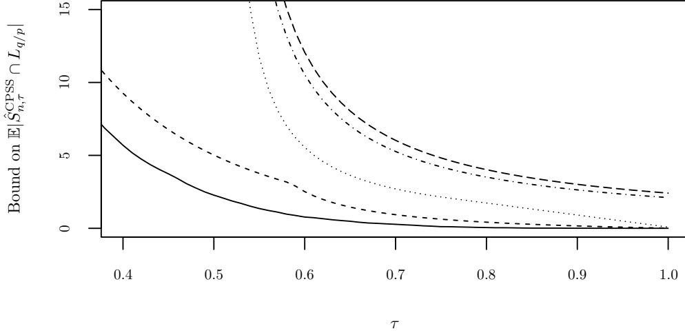
Fig. 2. Comparison of the bounds on \mathbb{E}|\hat{S}_{n,\tau}^{\text{CPSS}} \cap L_{q/p}| for different values of the threshold \tau : the original bound from Theorem 1 of Meinshausen and Bühlmann (2010) (long dashes), our worst case bound (dots and dashes), the unimodal bound (dots) and the r -concave bound (8) (short dashes). The solid line is the true value of \mathbb{E}|\hat{S}_{n,\tau}^{\text{CPSS}} \cap L_{q/p}| for a simulated example. In this case p = 1000 , q = 50 and the number of signal variables was 8.
