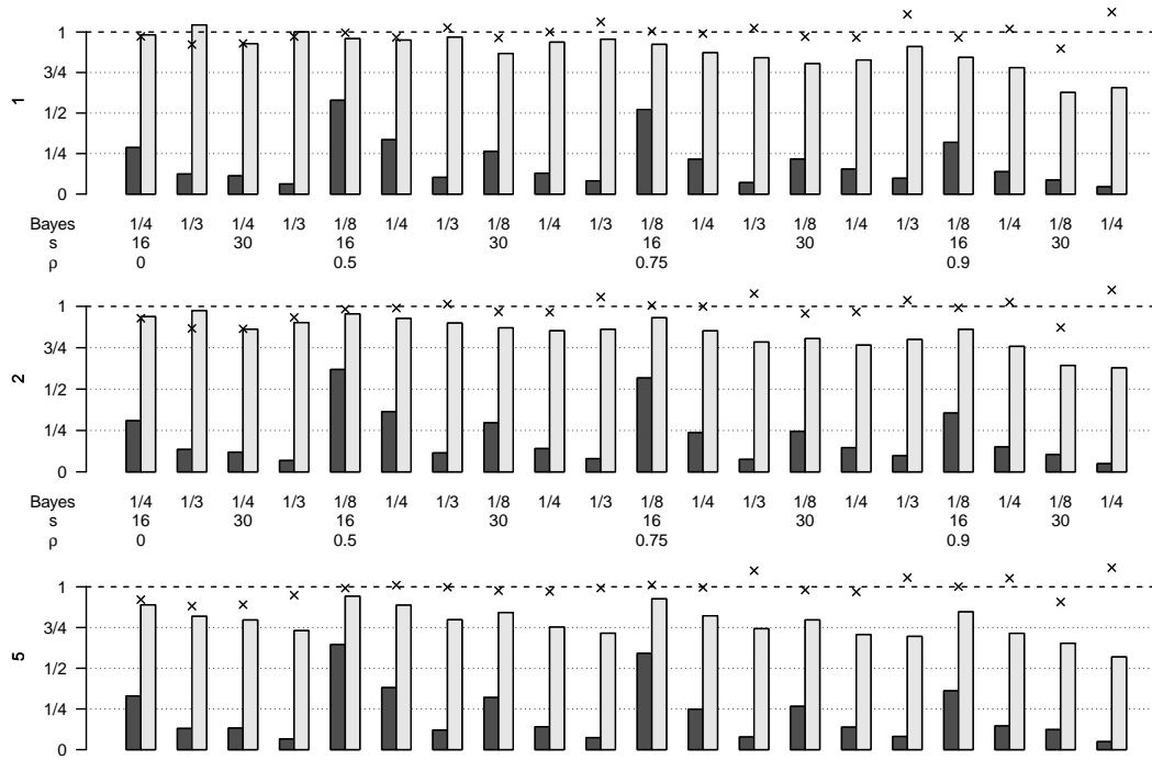
Fig. 7. As above but with with n = 500, p = 2000 .
