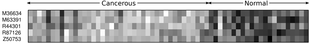
Fig. 9. A heatmap of the normalised, centered, log intensity values of the genes selected when we use the r -concave bound to choose \tau such that we control \mathbb{E}|\hat{S}_{n,\tau}^{\text{CPSS}} \cap L_{q/p}| \leq 0.5 .
