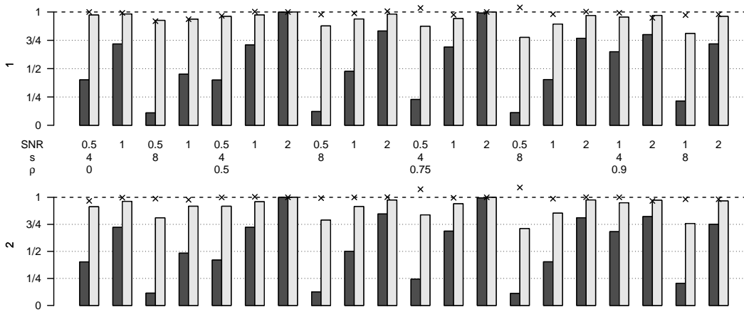
Fig. 4. Linear regression with n = 200 , p = 1000 . The black and grey bars correspond to the worst case and r -concave procedures respectively, with higher bars being preferred. The crosses correspond to a theoretical oracle-driven Lasso procedure (see the beginning of Section 4.1 for further details). The y -axis label gives the error control level l .
