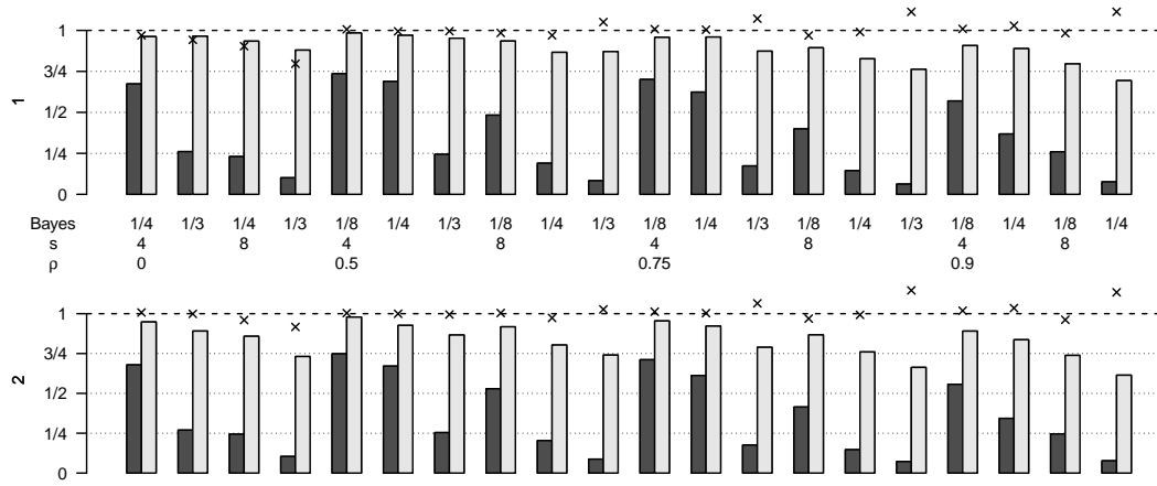
Fig. 6. As Figure 4 but with logistic regression (and n = 200, p = 1000 ).
