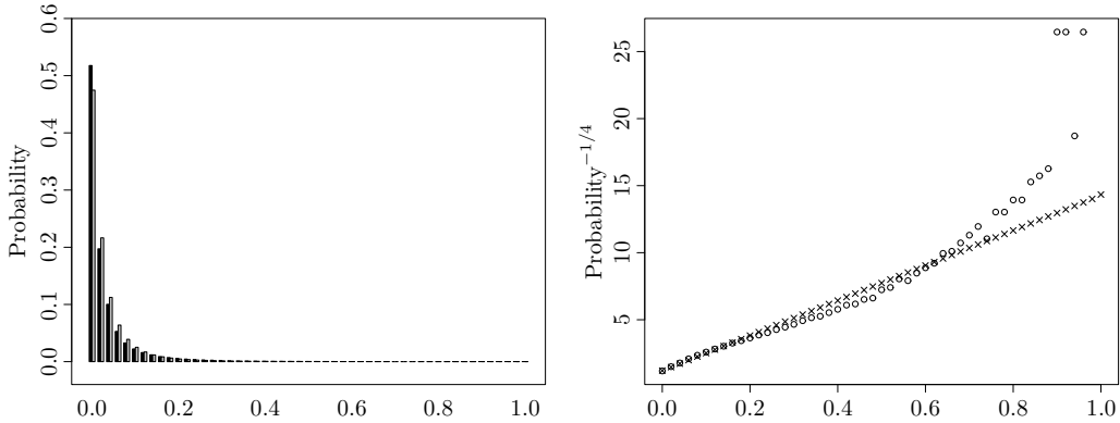
Fig. 3. A typical example of the probability mass function of \hat{\Pi}_{25}(k) for k \in L_{q/p} (black bars and circles), alongside the -1/4 -concave distribution (grey bars and crosses), which has maximum tail probability beyond 0.4.
