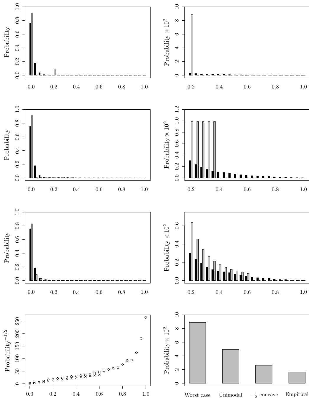
Fig. 1. Rows 1 to 3 show a typical example of the full probability mass function (left) and zoomed in from 0.2 onwards (right) of \Pi_{25}(k) for k \in L_{q/p} (black), alongside the unrestricted, unimodal and -1/2 -concave distributions respectively (grey), which have maximum tail probability beyond 0.2. This situation corresponds to selecting \tau = 0.6 . Bottom left: the observed mass function (circles) and the extremal -1/2 -concave mass function (crosses) on the x^{-1/2} scale. Bottom right: tail probabilities from 0.2 onwards for each of the distributions.
