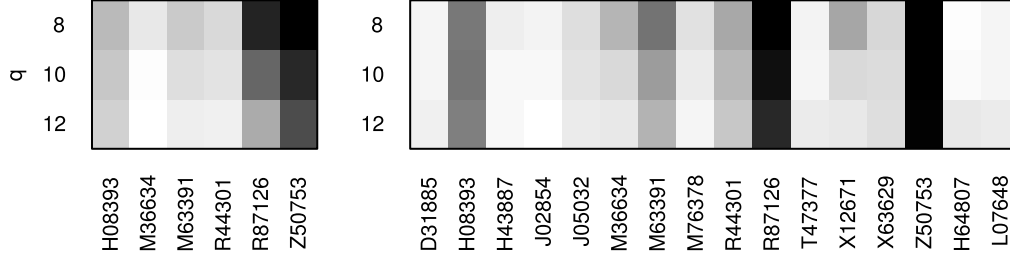
Fig. 8. For l = 0.1 (left) and l = 0.5 (right), we have plotted the proportion of times a gene was selected by our r -concave CPSS procedure for all genes which were selected at least 5% of the time among the 128 repetitions. Solid black means the gene was selected in every repetition, and white means it was never selected. Thus dark vertical lines indicate that the choice of q has little effect on the end result of CPSS.
