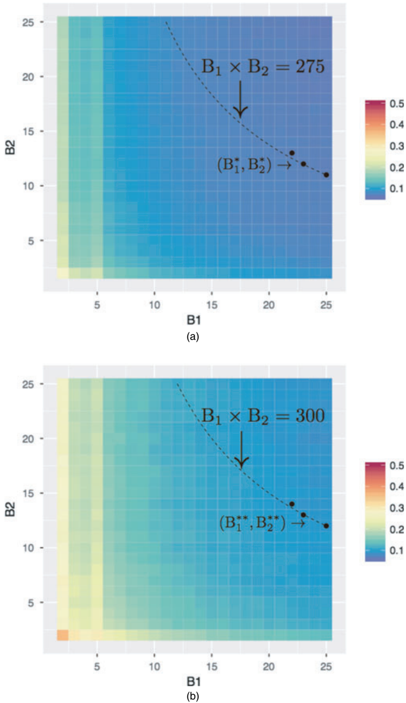
Fig. 7. Heat map of (a) the misclassification rate ( d = 5 ) and (b) CIS ( d = 5 ) under various values of (B_1, B_2) : the training data set of size 200 and the testing data set of size 1000 were generated following Section 6.1.2 of the paper; the k nn classifier is considered here; CIS is calculated by averaging the disagreement of two classifiers on the testing data with 100 replications
