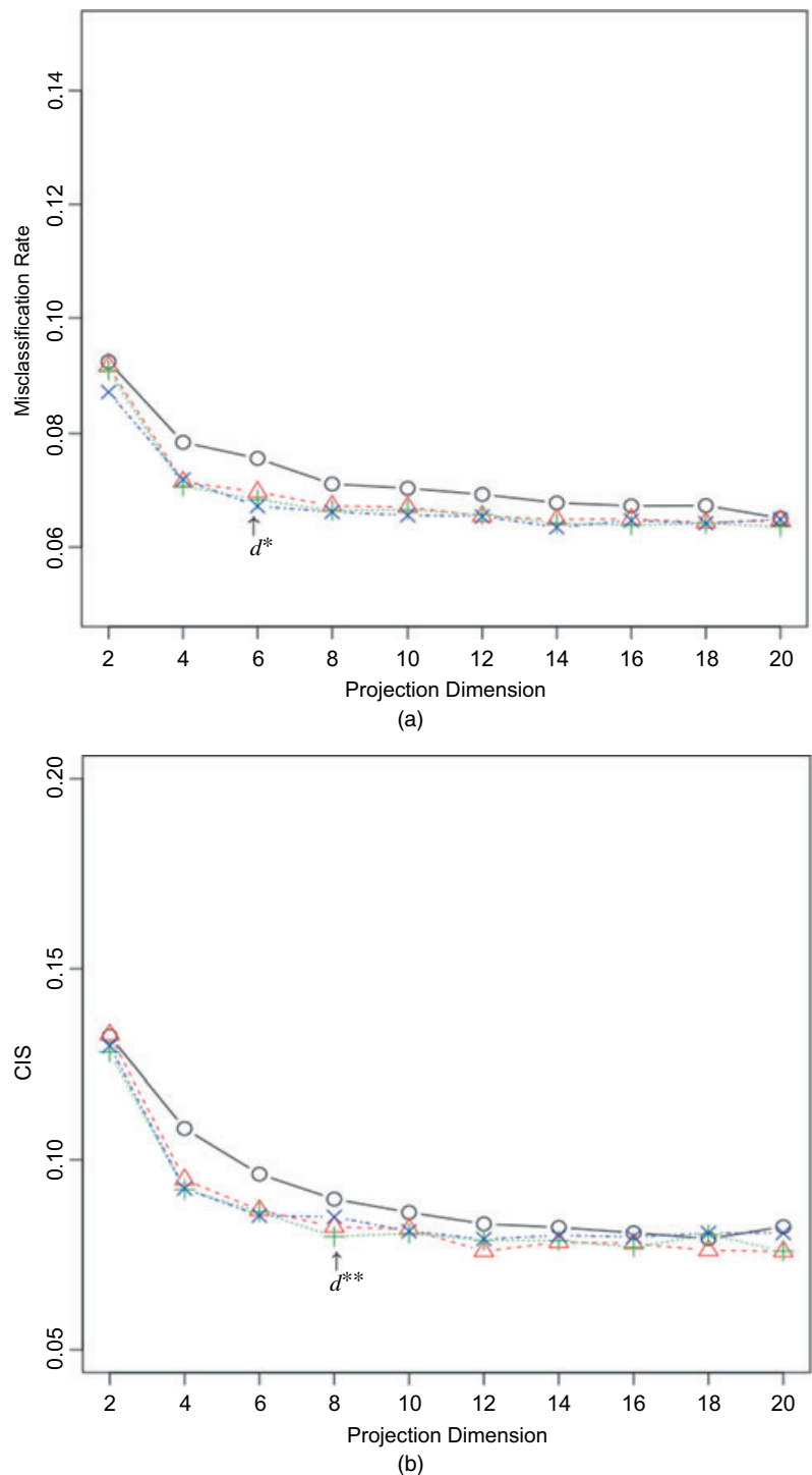
Fig. 8. Effect of projection dimension on (a) the misclassification rate and (b) CIS ( d ranges from 2 to 20, n = 200 and B_1 \times B_2 = 200 ; the knn classifier is considered here): \circ , B_1 = 20, B_2 = 10 ; \triangle , B_1 = 40, B_2 = 5 ; + , B_1 = 50, B_2 = 4 ; \times , B_1 = 100, B_2 = 2
