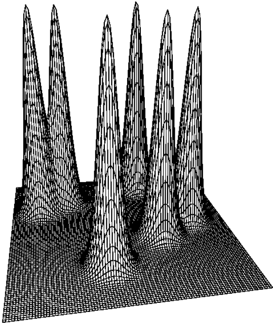
Fig. 1. Without any shape constraint on the class of densities, the likelihood function is unbounded, because we can take successively close approximations to a mixture of n 'spikes' (one on each X_i ).
