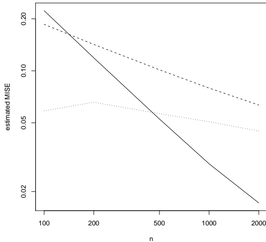
Fig. 6. MISE, d = 2 , Bivariate uniform/Beta density. The solid line is the LogConcDEAD estimate, the dashed line the plug-in kernel estimate, and the dotted line the Abramson kernel estimate.
