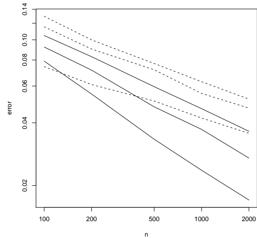
Fig. 9. Error for the highest density regions. The solid lines are the LogConcDEAD estimates; the dashed lines are the kernel estimates. The lowest lines are the 25% HDR, the middle lines are the 50% HDR and the highest lines are the 75% HDR.
