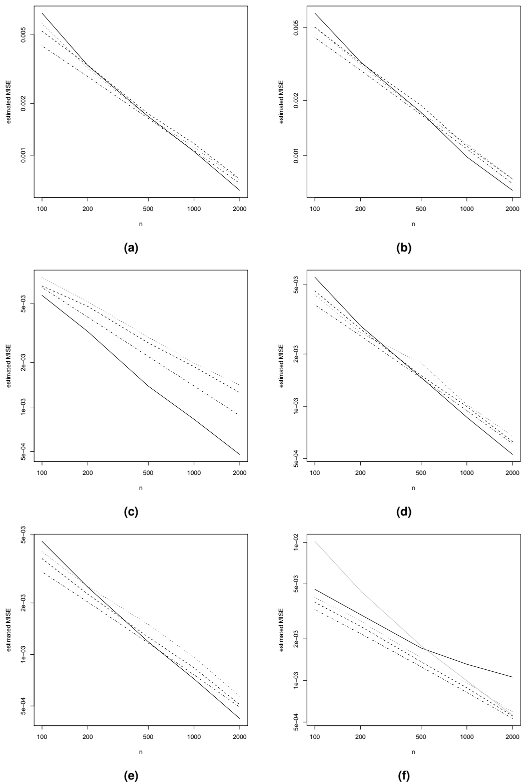
Fig. 4. MISE, d = 2 . The solid line is the LogConcDEAD estimate, the dashed line the plug-in kernel estimate, the dotted line the Abramson kernel estimate and the dot-dashed line the MISE-optimal bandwidth kernel estimate. The grey line (density f only) is for a 2-component log-concave mixture.
