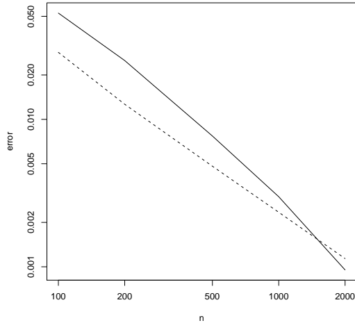
Fig. 8. MSE for the differential entropy estimates for density (c) and d = 2 . The solid line is the Log-ConcDEAD estimate; the dashed line is a kernel estimate.
