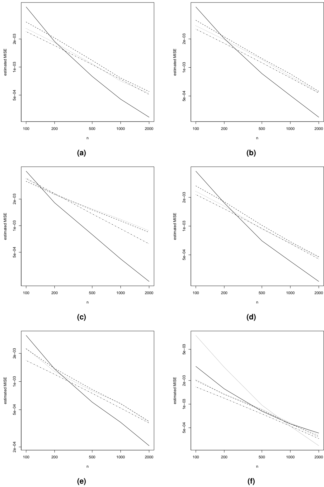
Fig. 5. MISE, d = 3 . The solid line is the LogConcDEAD estimate, the dashed line the plug-in kernel estimate, the dotted line the Abramson kernel estimate and the dot-dashed line the MISE-optimal bandwidth kernel estimate. The grey line (density f only) is for a 2-component log-concave mixture.
