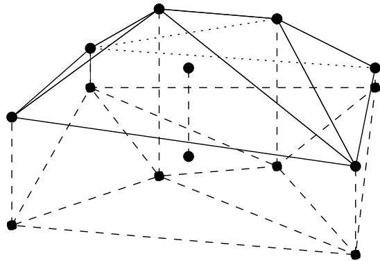
Fig. 2. The 'tent-like' structure of the graph of the logarithm of the maximum likelihood estimator for bivariate data.
