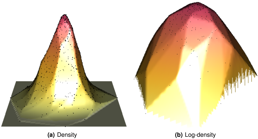
Fig. 3. Log-concave maximum likelihood estimates based on 1000 observations (plotted as dots) from a standard bivariate normal distribution.
