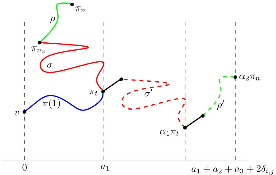
Fig. 1 Two images of v_{i,j} are introduced in order to make the required connections. These extra connections are drawn as black straight-line segments, and each has weight \theta_{i,j} , \ell -length s_{i,j} , and span \delta_{i,j}
