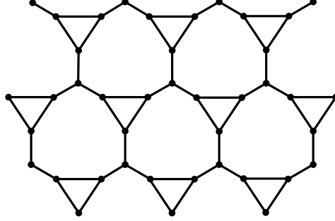
FIGURE 2.2. The lattice \tilde{\mathbb{H}} derived from the hexagonal lattice \mathbb{H} by applying the Fisher transformation at alternate vertices. Its connective constant \tilde{\mu} is the root of the equation x^{-3} + x^{-4} = 1/(2 + \sqrt{2}) .
