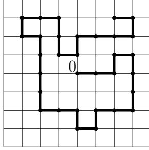
FIGURE 1.1. A SAW from the origin of the square lattice.
