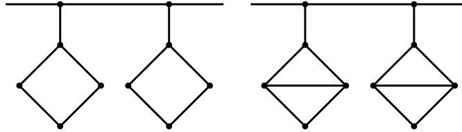
FIGURE 4.2. The pair G, \overline{G} . The graphs are extended in both directions. Each graph is quasi-transitive with connective constant 1, and the second is obtained from the first by a quasi-transitive addition of edges.
