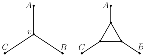
FIGURE 2.1. The Fisher triangulation of the star.
