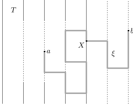
FIGURE 6. The Simon inequality. The separating set T is drawn with solid black lines, and the backbone \xi with a grey line.
