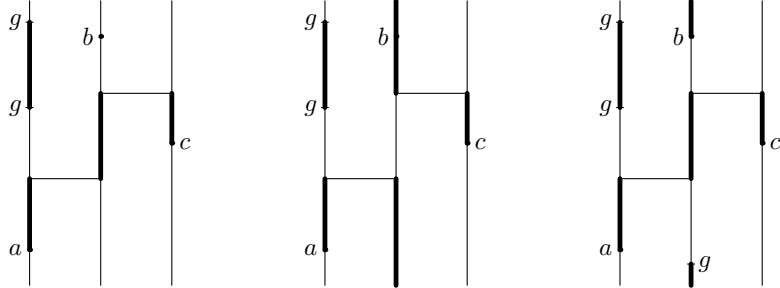
FIGURE 1. Three examples of colourings for given B \in \mathcal{B} , G \in \mathcal{F} . Points in G are written g . Thick line segments are ‘odd’ and thin segments ‘even’. In this illustration we have taken K_v = \mathbb{S} for all v . Left and middle : two of the six possible colourings when the sources are a, c . Right : one of the possible colourings when the sources are a, b, c .
