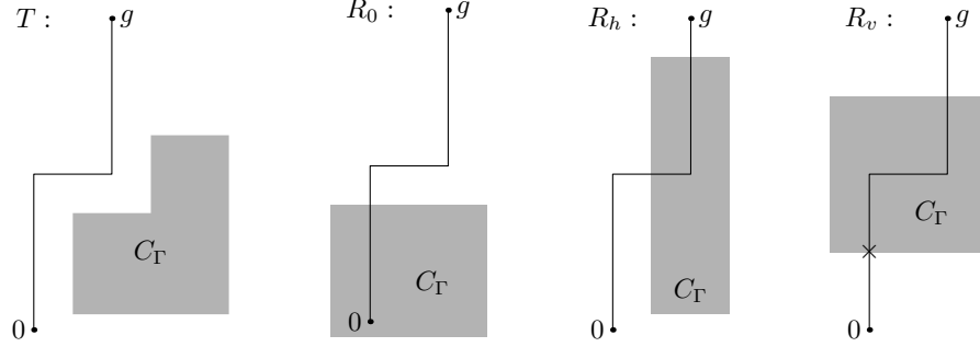
FIGURE 7. Illustrations of the four possibilities for \xi \cap C_\Gamma . Ghost-bonds in \psi^{0\Gamma} are labelled g . The backbone \xi is drawn as a solid black line, and C_\Gamma as a grey rectangle.
