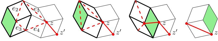
Fig. 6.7 Three star–triangle transformations contributing to \Sigma_{j+1} , from left to right. The dashed edges are closed, the bold passages are open. The first and last passages occur with probability 1, and the second with probability p_{e_1}p_{e_4}/(1-p_{e_1})(1-p_{e_4}) .
