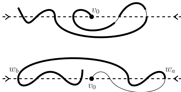
FIGURE 3. Two cases in the proof of \mu \leq \mu^B for undirected non-unimodular graphs: (i) the walk w (solid) has few intersections with the right half of the quasi-geodesic (dashed); (ii) w has many intersections with both halves of the quasi-geodesic. In both cases, each thickened portion of w is backward extendable.
