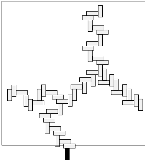
Fig. 7.10. Illustrations of the block construction for the proof of Theorem 7.35 presented in [50]. The grey regions contain open paths joining the black ‘inlet’ to the three ‘outlets’. The fundamental building block is a rectangle rather than a square. We have no control of the aspect ratio of this rectangle, and consequently two cases with somewhat different geometries need to be considered. Compare with Figure 7.7.
