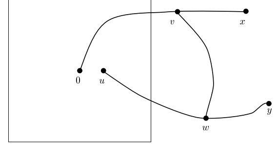
Fig. 8.1. If 0 \leftrightarrow x , u \leftrightarrow y , and x \leftrightarrow y off B , then there exist v, w \notin B such that there are disjoint open paths from x to v , from v to 0 , from v to w , from w to u , and from w to y .
