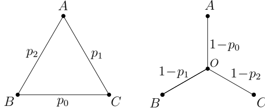
FIG 3.2. The star-triangle transformation
