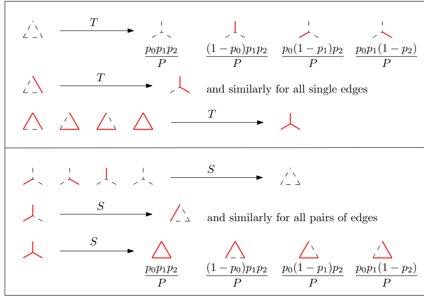
FIG 3.3. The random maps T and S and their transition probabilities, with P := (1-p_0)(1-p_1)(1-p_2) . Note that T(\omega) is deterministic for seven of the eight elements of \Omega ; only in the eighth case does T(\omega) involve further randomness. Similarly, S(\omega') is deterministic except for one special \omega' .
