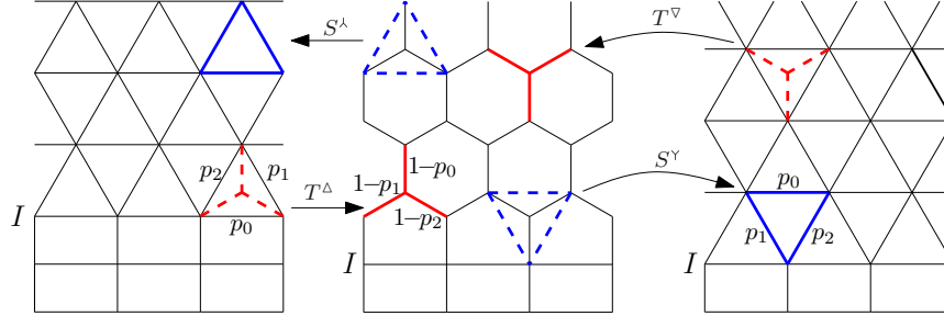
FIG 3.4. Transformations S^\lambda , S^\gamma , T^\Delta , and T^\nabla of mixed lattices. The transformations map the dashed stars/triangles to the bold stars/triangles. The interface-height decreases by 1 from the leftmost to the rightmost graph.
