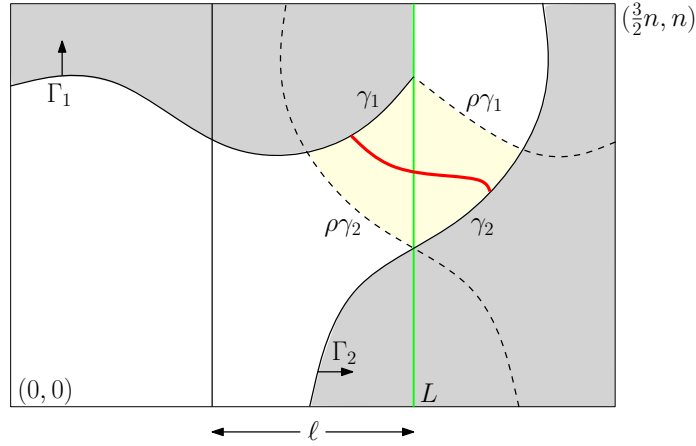
FIG 4.3. The path \Gamma_1 is the uppermost crossing of S_1 , and \Gamma_2 is the rightmost crossing of S_2 starting in \ell . The coloured region is framed by the \Gamma_i and their reflections in L . This is the simplest situation and there are more complex, depending on the \Gamma_i .
