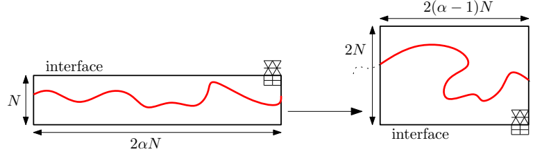
FIG 3.5. After N applications of S^Y \circ T^\Delta , a horizontal crossing of a rectangle of \mathbb{Z}^2 has been transformed into a crossing of a rectangle in \mathbb{T} with altered aspect-ratio.
