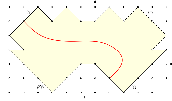
FIG 4.2. Under reflection \rho in the green line L , the primal lattice is mapped to the dual. The primal path \gamma_1 is on the left side with an endpoint abutting L , and similarly \gamma_2 is on the right. Also, \gamma_1 and \rho\gamma_2 are non-intersecting with adjacent endpoints as marked.
