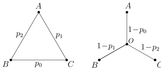
FIG 3.2. The star-triangle transformation
