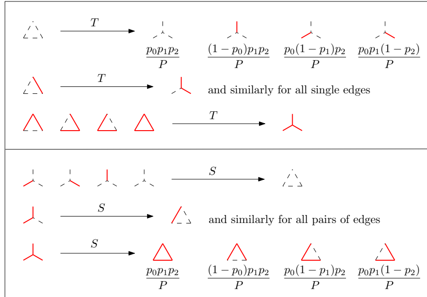
FIG 3.3. The ‘kernels’ T and S and their transition probabilities, with P := (1 - p_0)(1 - p_1)(1 - p_2) . Note that T(\omega) is deterministic for seven of the eight elements of \Omega ; only in the eighth case does T(\omega) involve further randomness. Similarly, S(\omega') is deterministic except for one special \omega' .
