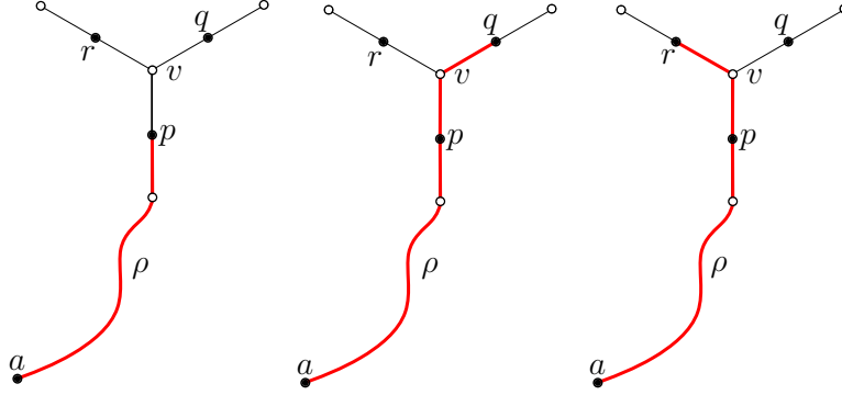
FIG 2.4. The left SAW, denoted \gamma_\rho , intersects the set \{p, q, r\} once only. The other two paths, denoted \gamma_q and \gamma_r , are extensions of the first.
