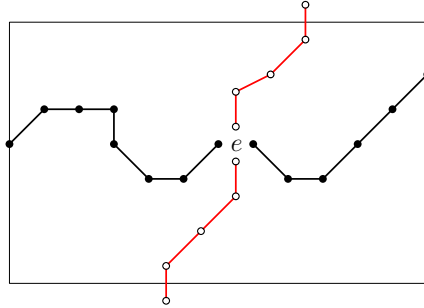
FIG 3.1. Primal and dual paths in the rectangle R . A black path is an open primal path, and a red path an open dual path. An edge e is pivotal for the box-crossing event if and only if there are four arms of alternating type from e to the boundary of the box.
