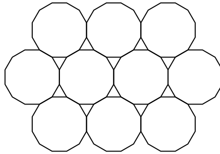
FIG 2.1. The Archimedean lattice (3, 12^2) is obtained by replacing each vertex of the hexagonal lattice by a triangle.
