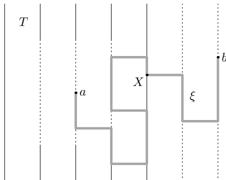
FIGURE 6. The Simon inequality. The separating set T is drawn with solid black lines, and the backbone \xi with a grey line.
