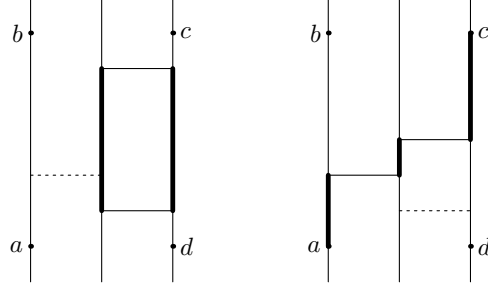
FIGURE 5. Switched configurations. Taking Q_1^{ac} , Q_2^{\emptyset} and \pi to be \psi_1^{ac} , \psi_2^{\emptyset} and \pi of Figure 4, respectively, this figure illustrates the ‘switched’ configurations R_1^{\emptyset} and R_2^{\emptyset} (left and right, respectively).
