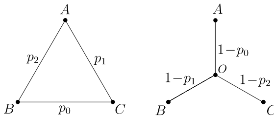
FIG. 3. The star–triangle transformation when \kappa_\Delta(\mathbf{p}) = 0 .
