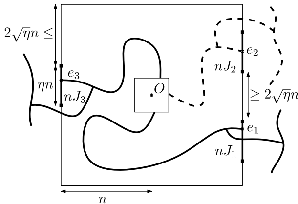
FIG. 9. The event A_\sigma^{\emptyset,J}(N, n) with \sigma = (1, 0, 1) and \eta -landing-sequence J . Each crossing \Gamma_i is an \eta -exterior-fence with exterior endpoint e_i \in nJ_i .
