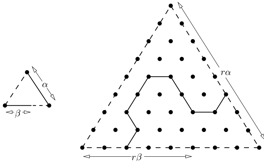
Fig. 2.3. An illustration of the triple (\gamma; \alpha, \beta) and of the event relevant to the probability \pi_r(\gamma; \alpha, \beta) .
