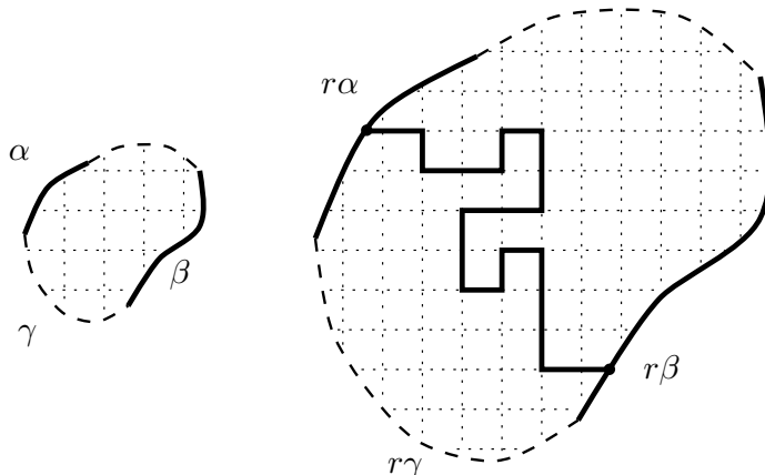
Fig. 2.1. An illustration of the event that r\alpha is joined to r\beta within r\gamma , in the case of bond percolation on \mathbb{Z}^2 .
