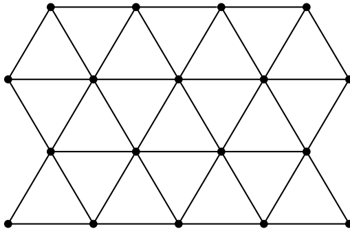
Fig. 2.2. Part of the triangular lattice.
