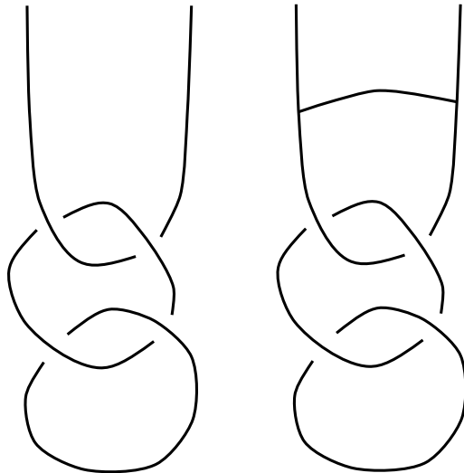
Fig. 4.2. The left graph is weakly but not strongly entangled; the right graph is both strongly and weakly entangled.
