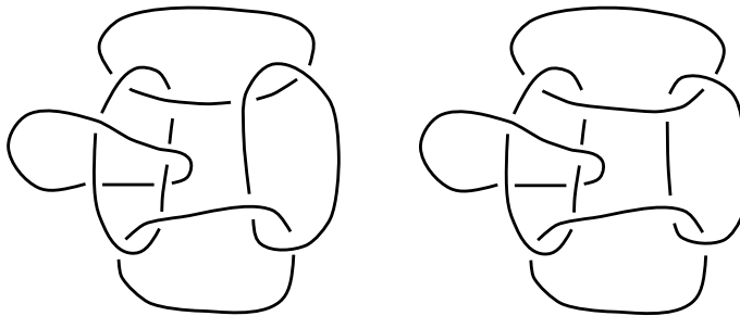
Fig. 4.1. The left graph is not entangled; the right graph is entangled.
