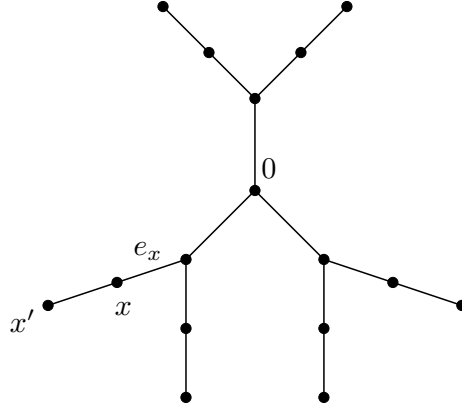
Figure 6.1. To each boundary vertex x of the first k ( = 2 ) generations of T'_m is attached a new edge [x, x'] .
