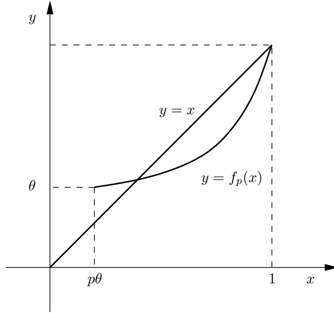
Figure 2.1. A sketch of the graphs of y = x and y = f_p(x) on the interval [p\theta, 1] . Whether or not there exists a root of \alpha = f_p(\alpha) other than at \alpha = 1 depends on the gradient of f_p at \alpha = 1 .
