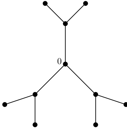
Figure 4.1. Part of the infinite binary tree T'_2 .
