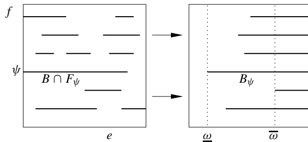
Figure 4.2. In the e/f -plane, we push every B \cap F_\psi as far rightwards along the fibre F_\psi as possible.
