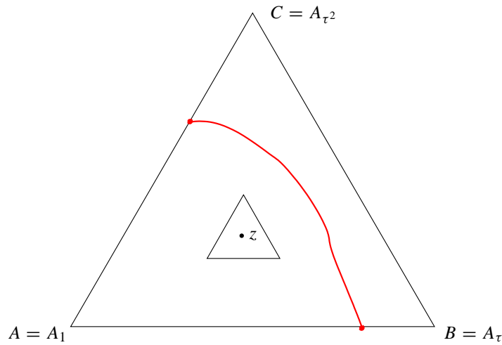
Figure 5.16. An illustration of the event E_1^n(z) , that z is separated from A_\tau A_{\tau^2} by a black path joining A_1 A_\tau and A_1 A_{\tau^2} .
