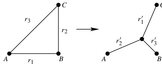
Figure 1.6. Edge-resistances in the star–triangle transformation. The triangle T on the left is replaced by the star S on the right, and the corresponding resistances are as marked.
