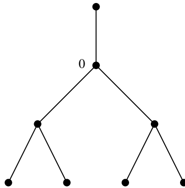
Figure 6.3. Part of the binary tree T_2 .
