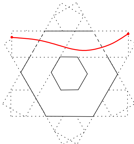
Figure 5.10. If each of six long rectangles are traversed in the long direction by black paths, then the intersection of these paths contains a black cycle within the annulus A_n .
